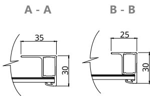
Frame Cross Section
